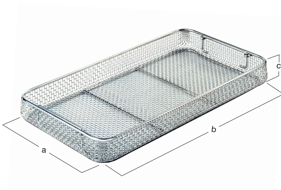
Siebkorb L Wire basket L
